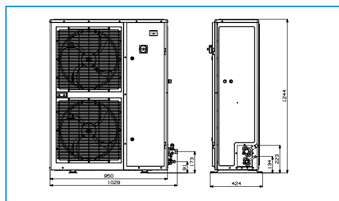
Agregaty dwuwentylatorowe
