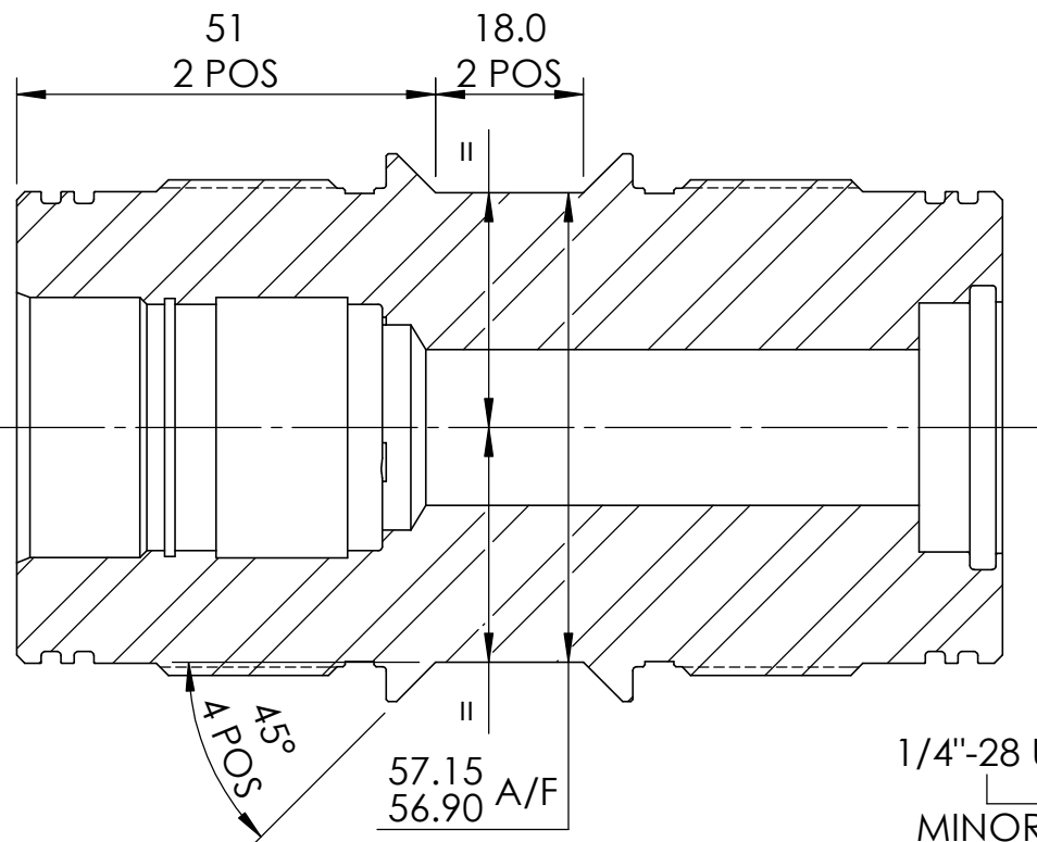
SECTION H-H
