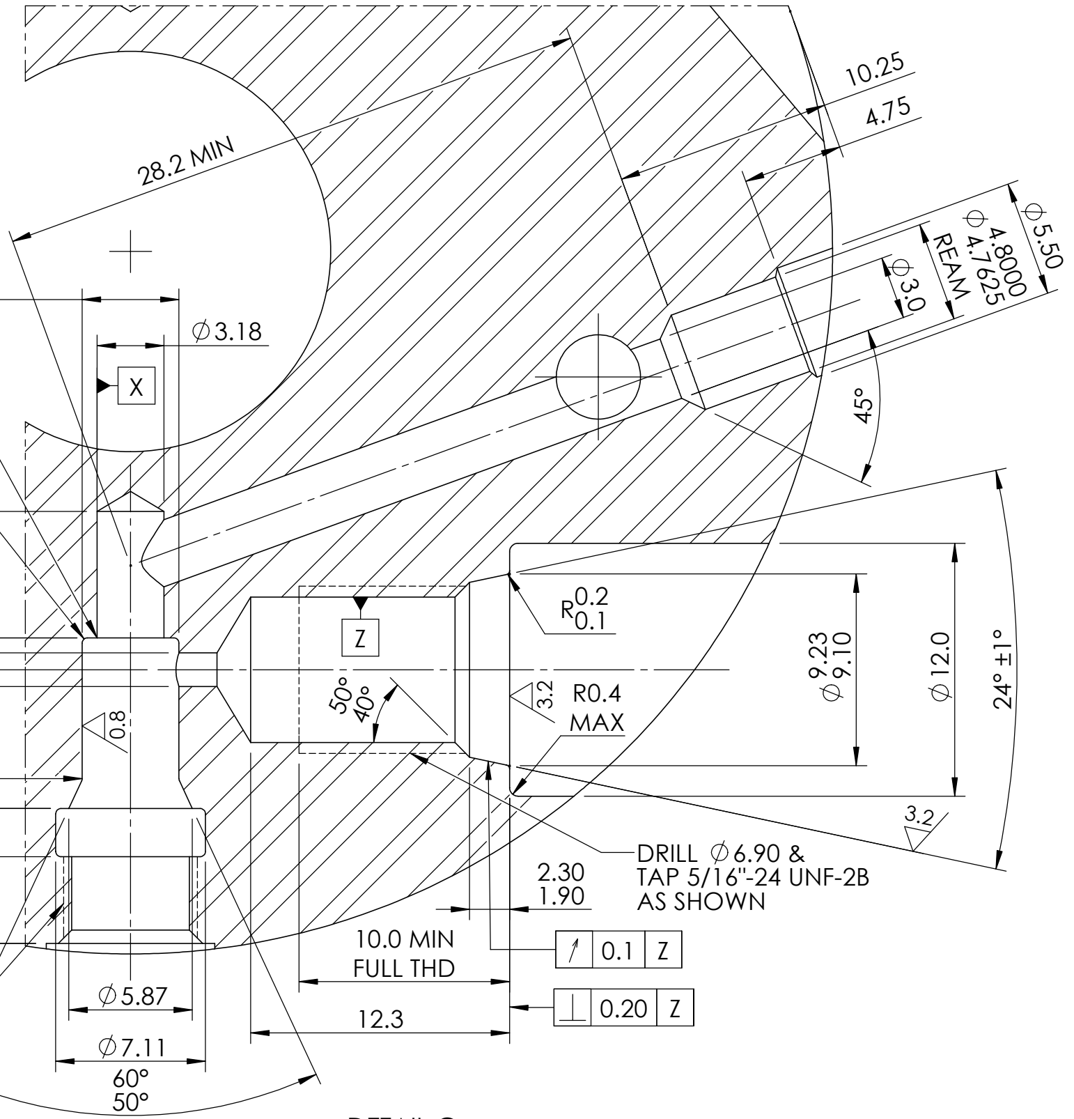
DETAIL G 1/4-28 UNF & 5/16-24 UNF PORT DETAILS TYP TO 2 POS
