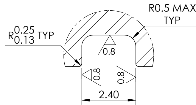
DETAIL B TYP 2 SEAL GROOVE DETAIL O-RING SIZE BS-034
